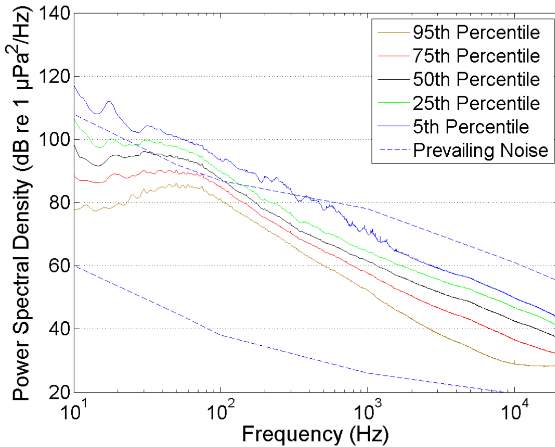
Figure 22: Percentile 1-min power spectral density levels (dB re 1 μPa 2 /Hz) for the summer 2011 deployment at HYWIND Control Station. The dashed lines are the 'Limits of Prevailing Noise' from the Wenz curves, Figure 3.
