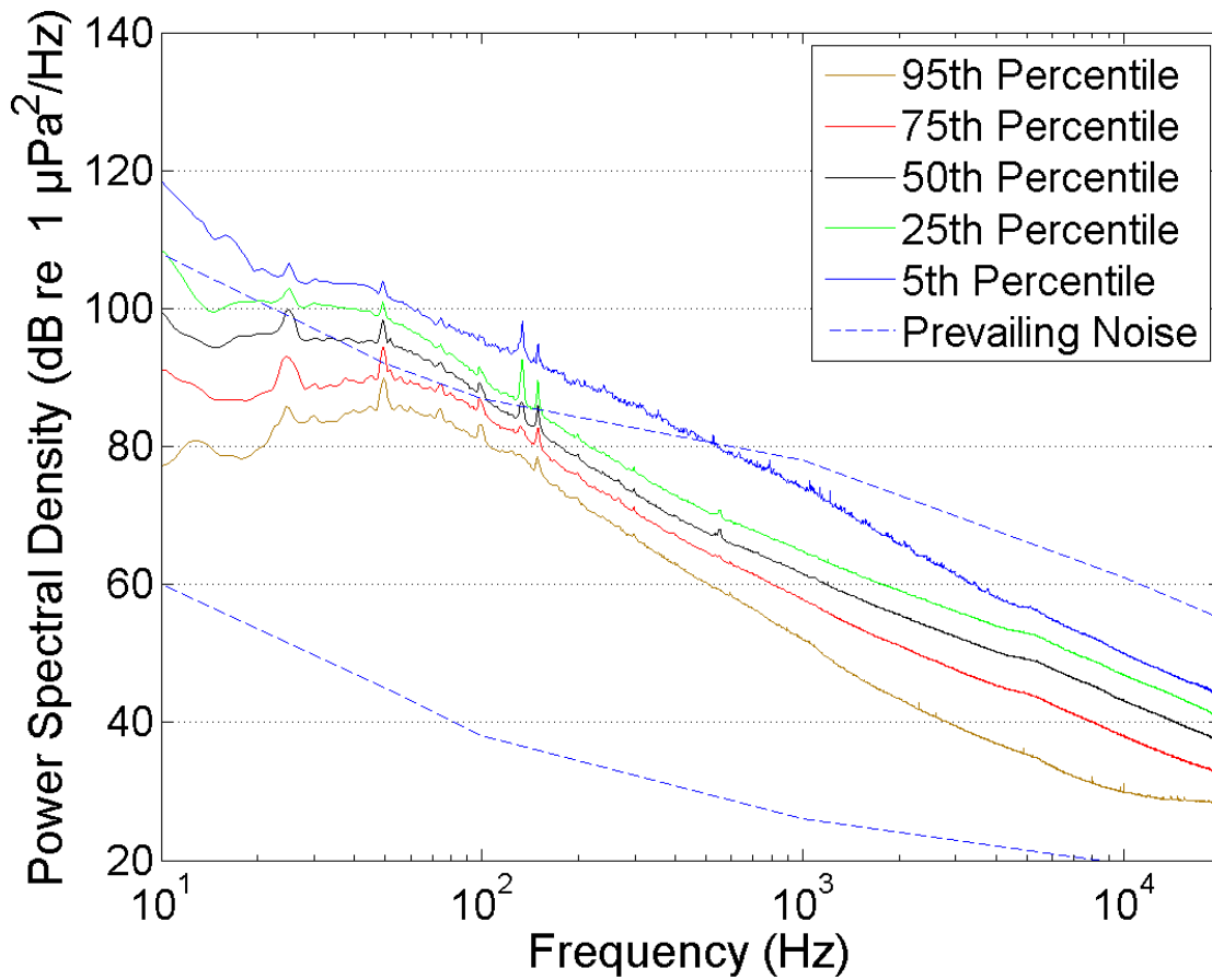
Figure 25: Percentile 1-min power spectral density levels (dB re 1 μPa 2 /Hz) for the summer 2011 deployment at HYWIND Monitoring Station. The dashed lines are the ‘Limits of Prevailing Noise’ from the Wenz curves, Figure 3.
