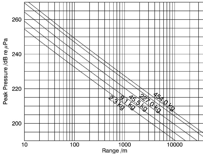
Figure 3. Peak pressures versus distance from detonations of the charge weights listed in Table 1, calculated with Eqs. 2 and 4.
