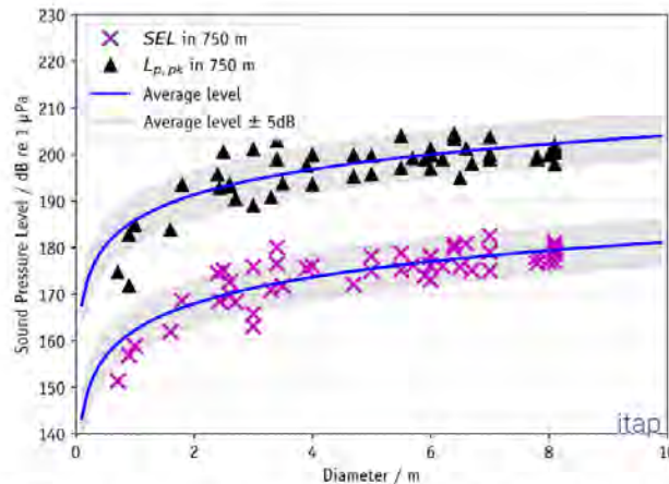
Figure 3: Measured zero-to-peak Sound Pressure Level ( L_{p, pk} ) and broad-band 5 % exceedance Sound Exposure Levels ( SEL_{0.05} ) at pile driving construction works at a number of offshore wind farms (OWFs) as function of the pile diameter.
