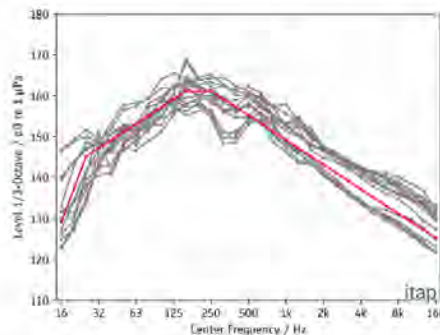
Figure 4: The model spectrum (red) estimated for piling noise, based on different measuring data (grey: measuring data) for monopiles.
