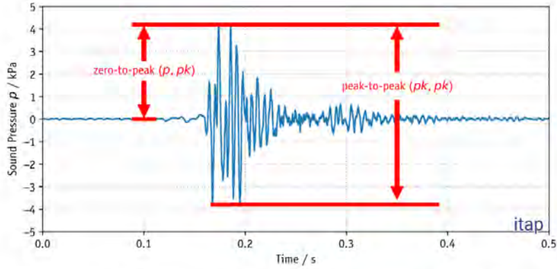
Figure 1: Typical measured time signal of underwater sound due to pile driving in a distance of several hundreds of meters.
