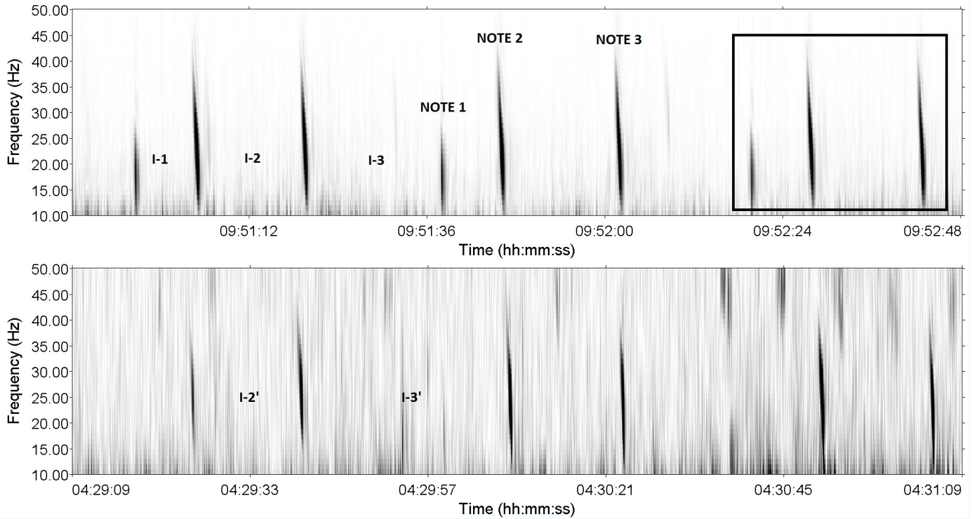
FIG. 4. Segments of fin whale songs recorded at station PL50 in the northeastern Chukchi Sea (top) on 15 September 2007 and (bottom) on 3 October 2010. The box shows a song unit, called a triplet. Notes 1, 2, and 3 represent the three components of a triplet. I-1, I-2, and I-2' refer to the intervals between consecutive notes; I-3 and I-3' refer to the interval between two consecutive triplet units. Note 1 is not present in the 2010 song. The spectrogram was generated using a Reisz window with 1 Hz frequency resolution, a frame size of 0.128 s, and a time step of 0.064 s. Time on the x-axis is in hours, minutes, and seconds (hh:mm:ss).
