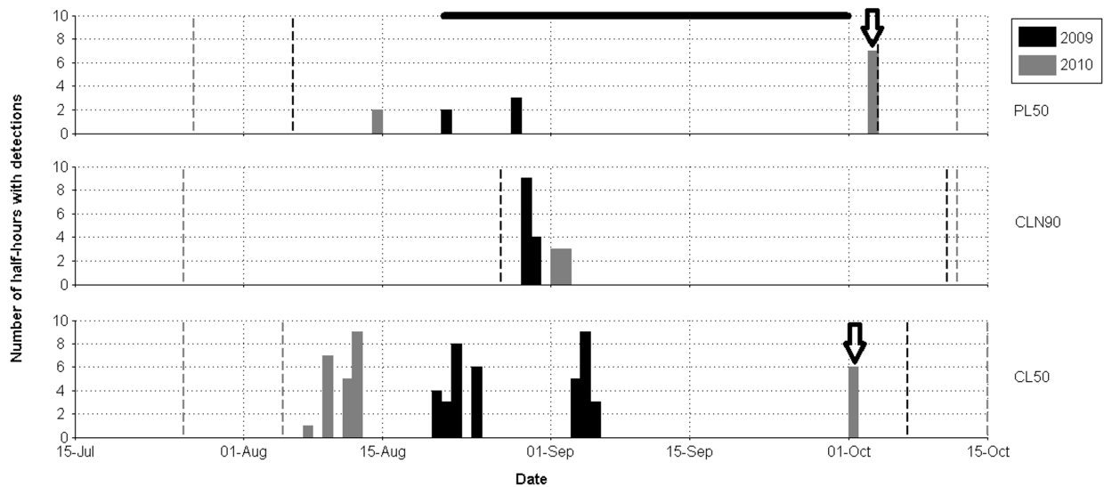
FIG. 6. Daily number of half-hours with manual fin whale detections based on the analysis of 5% of acoustic data recorded in the Chukchi Sea from late July to mid-October in 2009 (black) and 2010 (grey). Only the stations where fin whale calls were recorded are shown. Vertical dashed lines indicate recorder deployment and retrieval. The black bar represents the duration of the seismic survey detected at CLN90 and PL50 in 2010. The arrows mark the first song detection.
