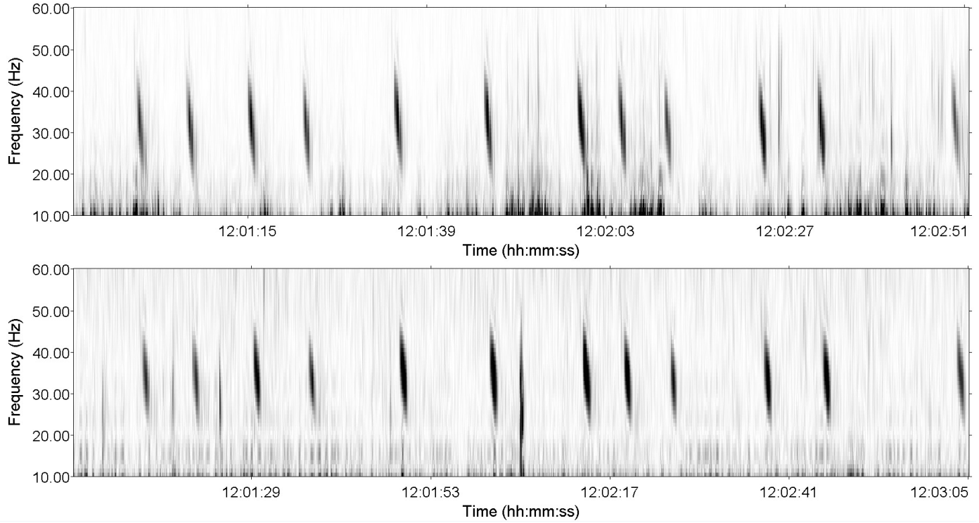
FIG. 3. A fin whale irregular pulse sequence recorded at CL35 (top) and CL50 (bottom) on 11 September 2007. These recorders were 28 km apart. The spectrogram was generated using a Reisz window with 1 Hz frequency resolution, a frame size of 0.128 s, and a time step of 0.064 s. Time on the x-axis is in hours, minutes, and seconds (hh:mm:ss).
